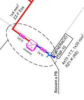
DETALL INVERSOR
